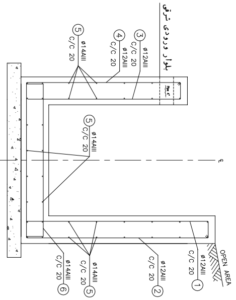
برش D-D NO SCALE REINFORCEMENT
